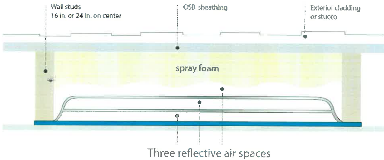
Figure 2 – HY-Fi Hybrid Wall with Spray Foam Illustration
