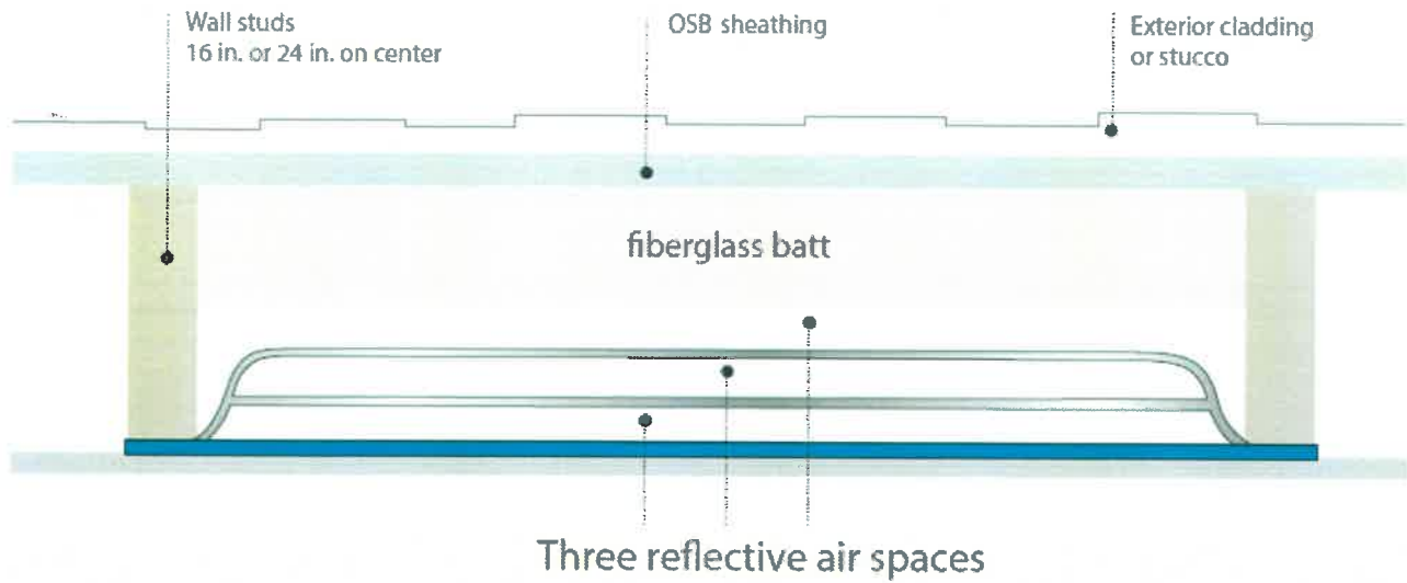
Figure 1 – HY-Fi Hybrid Wall with Fiberglass Batt Illustration
